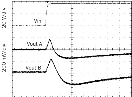
SMRT2812D Representative of Dual Output Line Transient
