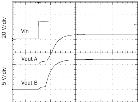
SMRT2812D Representative of Dual Turn On Delay
