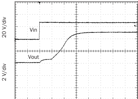
Full resistive load, 28 Vin
