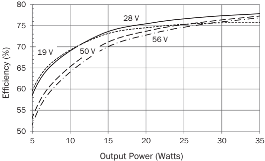
SMRT2812S Efficiency FIGURE 14
