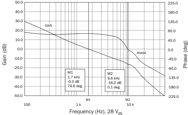
SMRT2812S Gain Phase FIGURE 15
