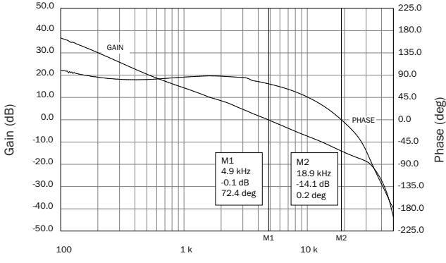
SMRT2805S Gain Phase FIGURE 11
