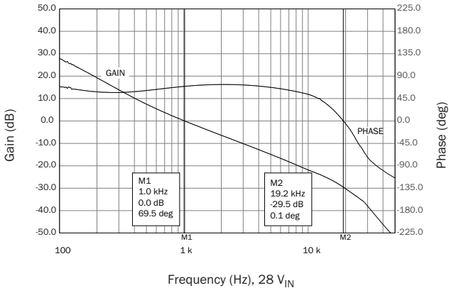
SMRT283R312T Gain Phase, +Aux Representative of all 12 V +Aux models FIGURE 45
