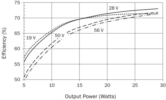
SMRT28507T Efficiency FIGURE 47
