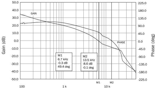
SMRT2812D Gain Phase FIGURE 30
