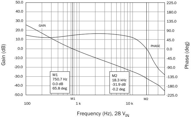
SMRT28515T Gain Phase, +Aux Representative of all 15 V +Aux models FIGURE 52
