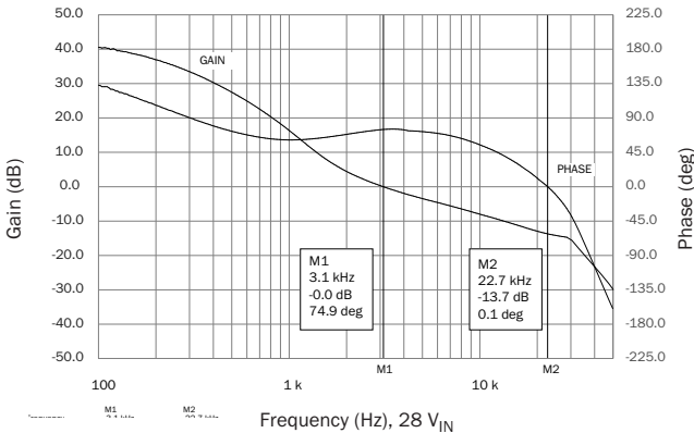
SMRT283R312T Gain Phase, Main Vout Representative of all 3.3 V Main models FIGURE 44
