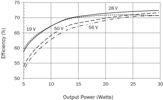
SMRT283R312T Efficiency FIGURE 43
