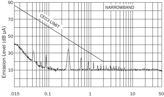
Frequency (MHz), 28 V_{IN} SMRT Single MIL-STD-461C, CE03 FIGURE 18
