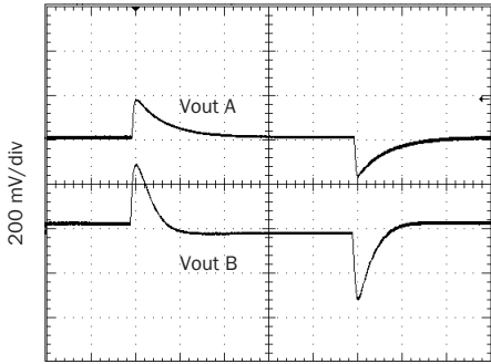
SMRT2812D Representative of Dual Output Load Transient
