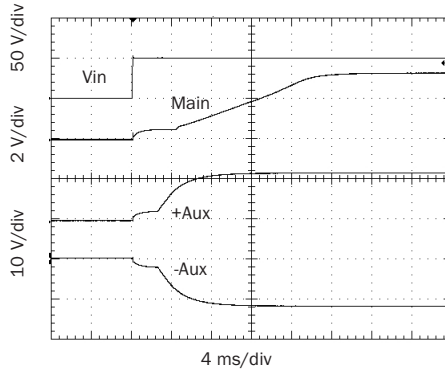
Full resistive load, 50 Vin SMRT283R312T Representative of Triple Output Turn On Delay FIGURE 62
