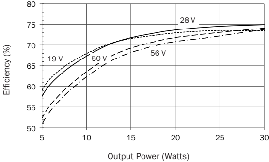
SMRT28512T Efficiency FIGURE 49
