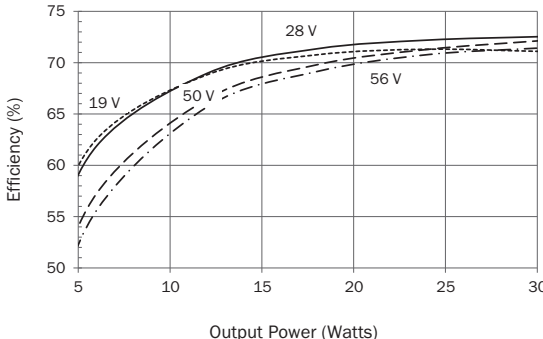
SMRT2805S Efficiency FIGURE 10
