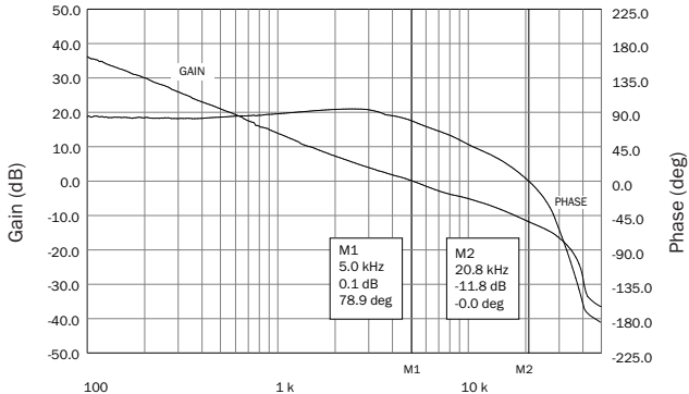
SMRT2805D Gain Phase FIGURE 28
