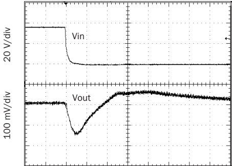
Vin 56 to 19 V, full resistive load
