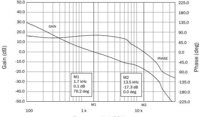
SMRT288R7S Gain Phase FIGURE 13
