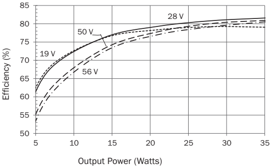
SMRT2815S Efficiency FIGURE 16
