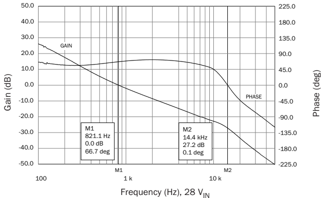
SMRT2815S Gain Phase FIGURE 17
