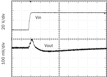
Vin 19 To 56 V, full resistive load
