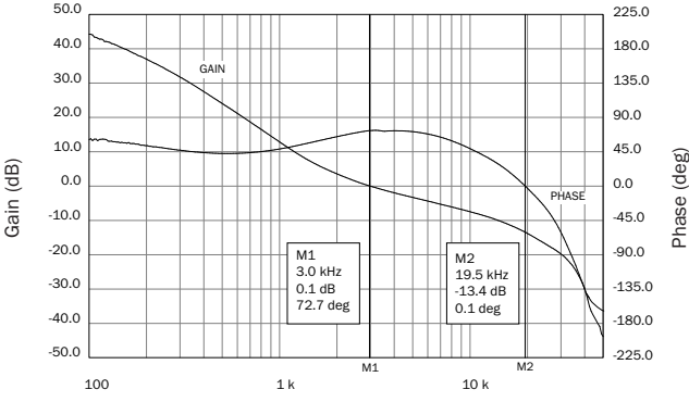
SMRT283R3S Gain Phase FIGURE 9
