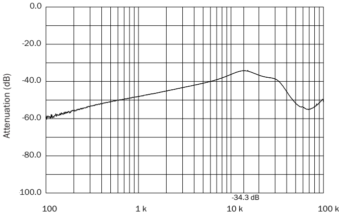
Frequency (Hz), 28 V_{IN} SMRT Single Audio Rejection FIGURE 20
