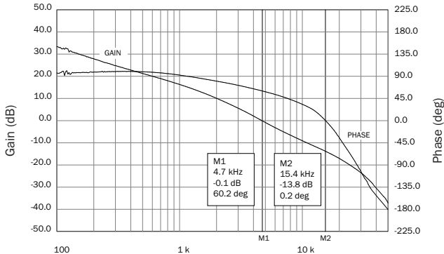
SMRT2815D Gain Phase FIGURE 32
