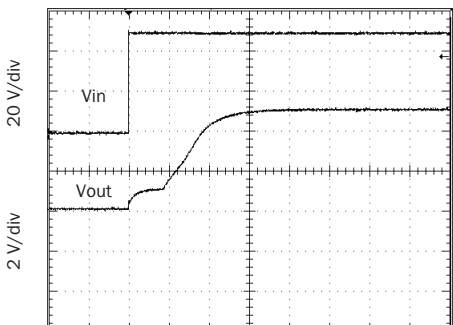
Full resistive load, 50 Vin
