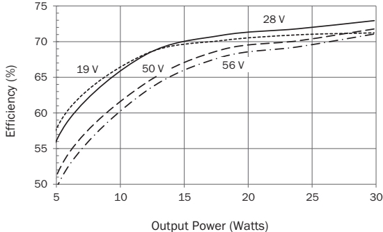
SMRT283R315T Efficiency FIGURE 46
