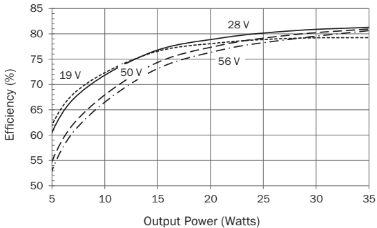
SMRT2815D Efficiency FIGURE 31
