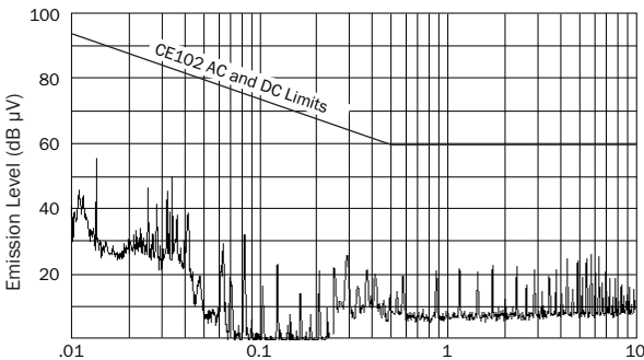
Frequency (MHz), 28 V_{IN} SMRT Single MIL-STD-461 D-F, CE102 FIGURE 19
