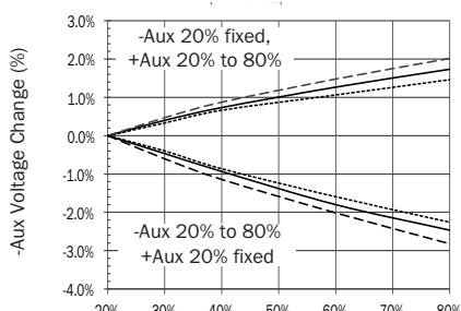
+Aux Load (%), 28 V_{IN} ..... -55 °C — 25 °C - -125 °C SMRT28515T Cross Regulation FIGURE 65
